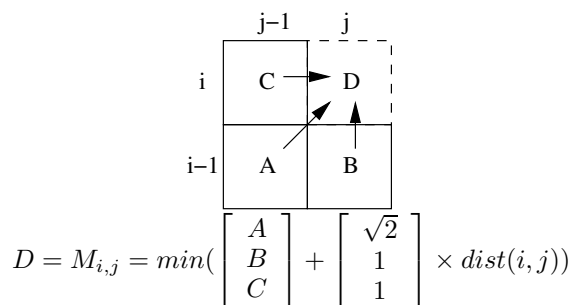
Figure 3: Calculation pattern for cell (i, j)
