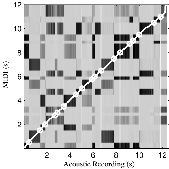
Figure 4: The optimal alignment path is shown in white over the similarity matrix of Figure 2; the little circles on the path denote the mapping of note onsets.
