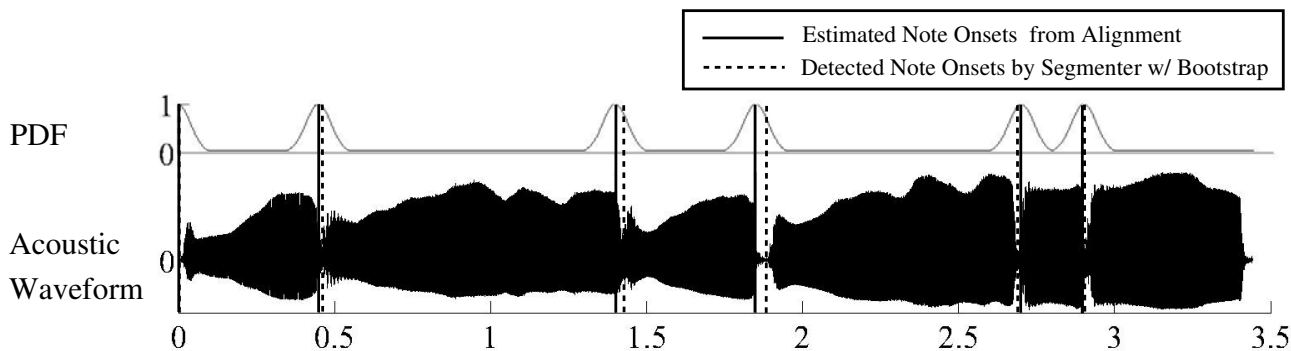
Figure 7: Note segmentation results on the same music content as in Figure 6. Note that the note onsets detected by the segmenter with bootstrapping are not exactly the same as the ones estimated from alignment. This is best illustrated on the note boundary around 1.8 seconds.
