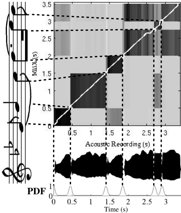
Figure 6: PDF generated from the alignment of a snippet, which is a phrase of the music content in Figure 2.
