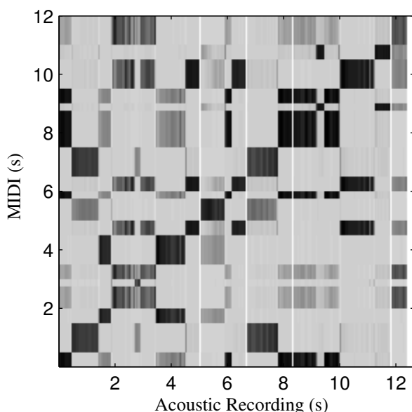
Figure 2: Similarity Matrix for the first part in the third movement of "English Suite" composed by R. Bernard Fitzgerald. The acoustic recording is the trumpet performance by the second author.
